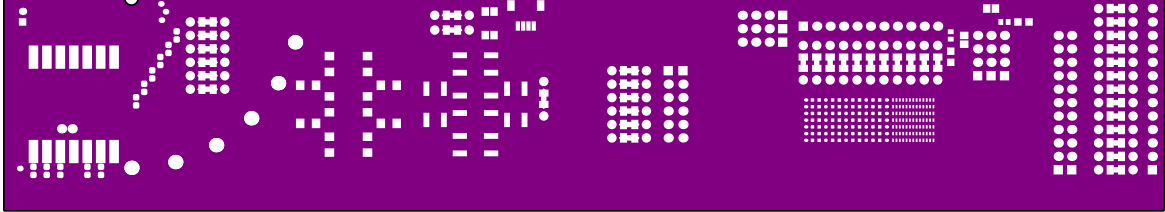
Top Solder (Scale 1:1.43)
